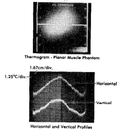
Fig. 11. Surface heating pattern.
