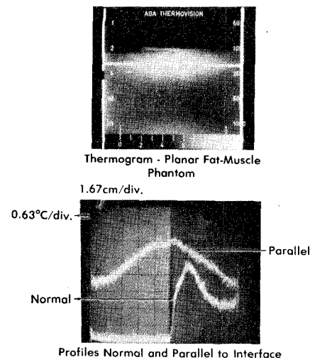
Fig. 10. Internal heating pattern 3.8 cm from center of applicator.
