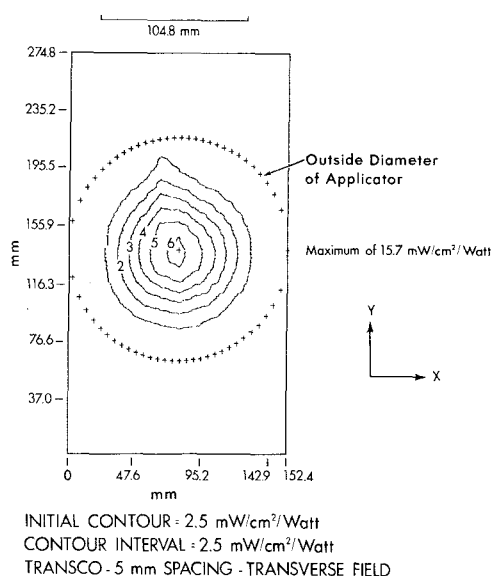
Fig. 6. Plot of isopower density contours of transverse field.
