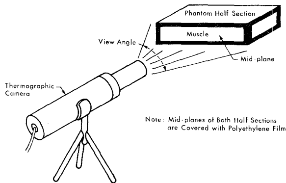
Fig. 8. Experimental setup.
