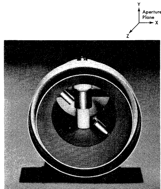
Fig. 2. Internal view of applicator with coaxial input probe and phasing post.
