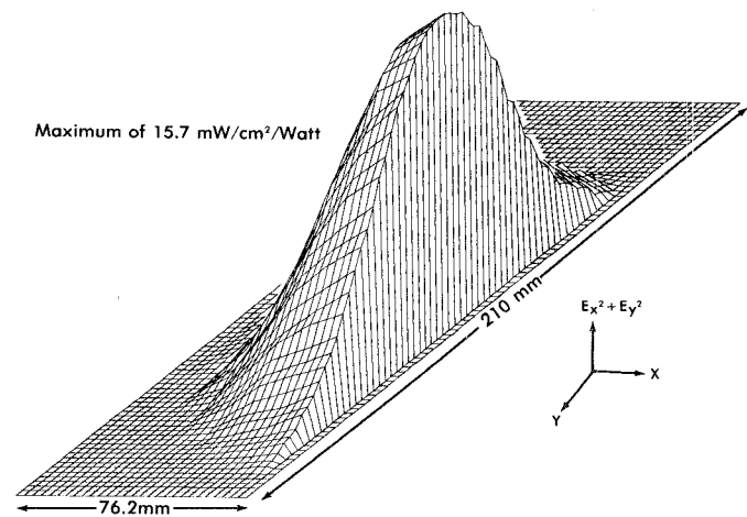
Fig. 5. Plot of half section of transverse field.
