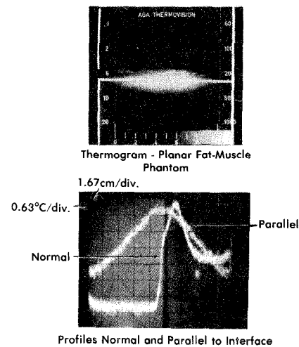
Fig. 9. Internal heating pattern at center of applicator.
