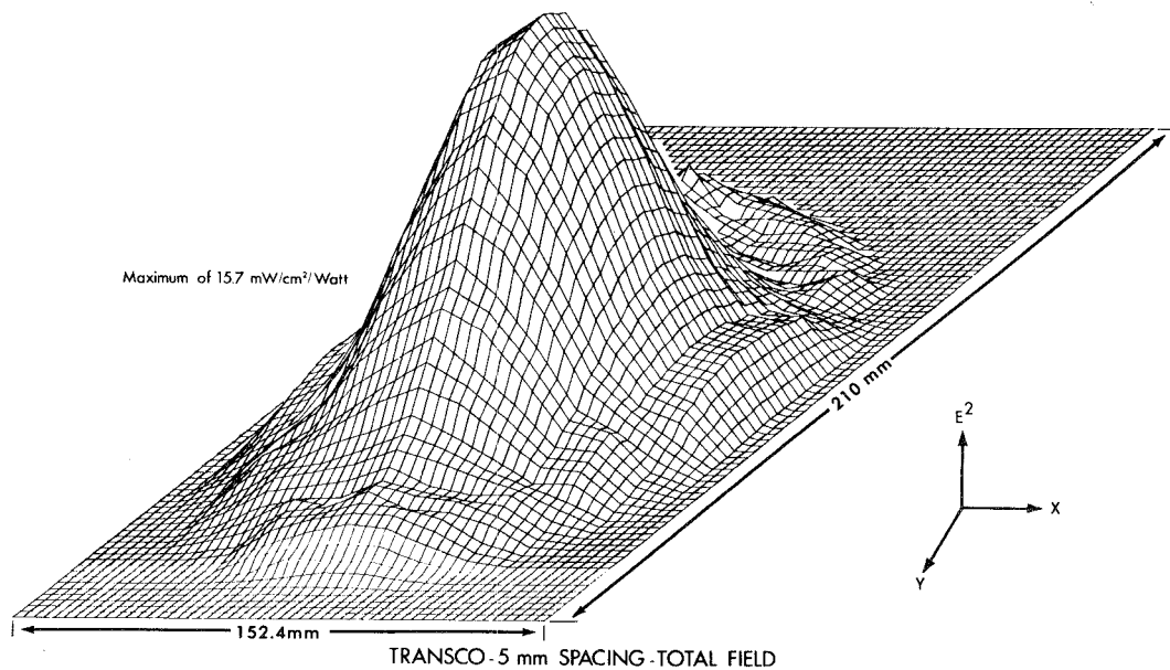
Fig. 3. Plot of total field.
